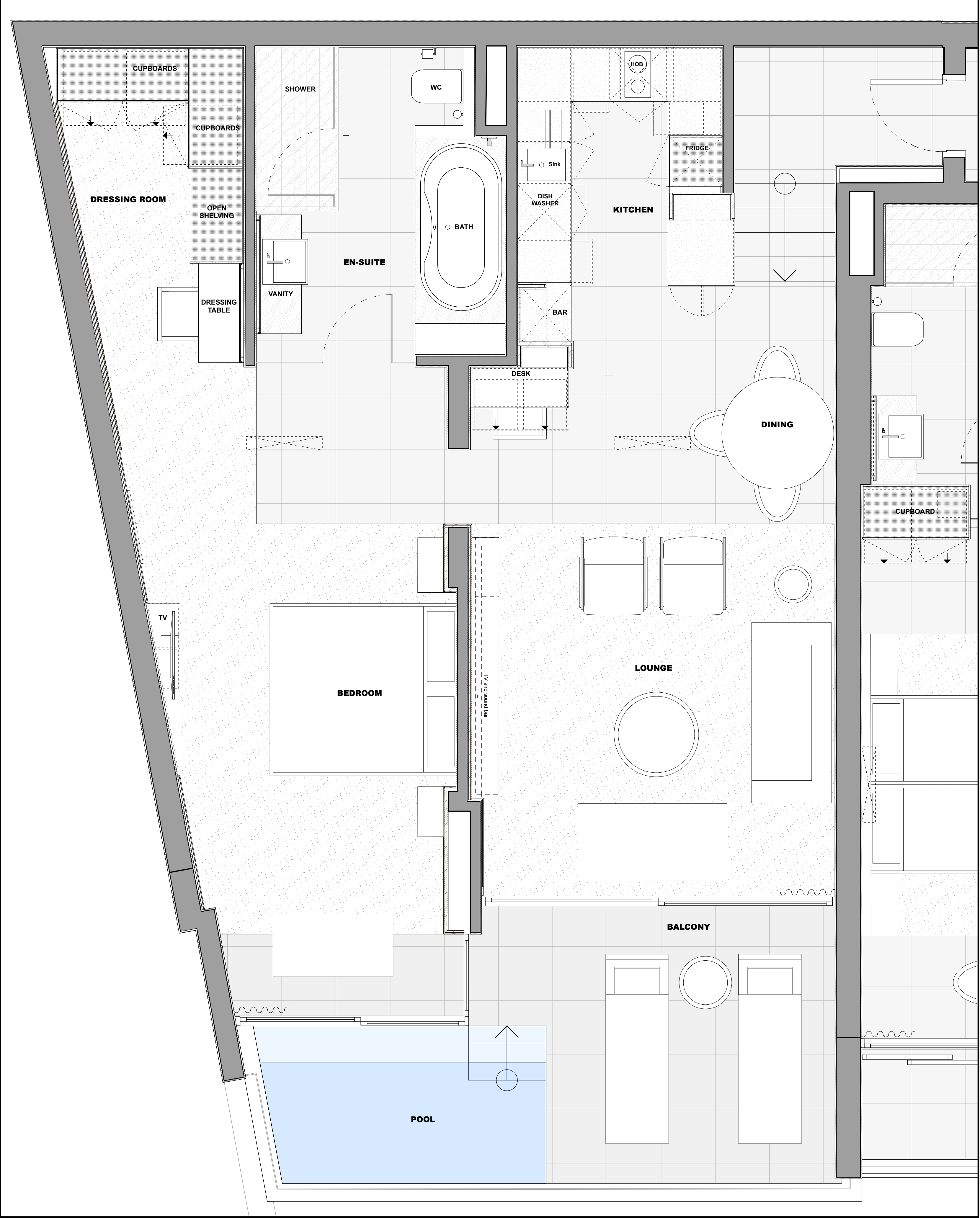
SUITE 205 | INTERNAL AREA: 89,08 SQM. BALCONY AREA: 16,27 SQM. TOTAL AREA: 105,35 SQM.
